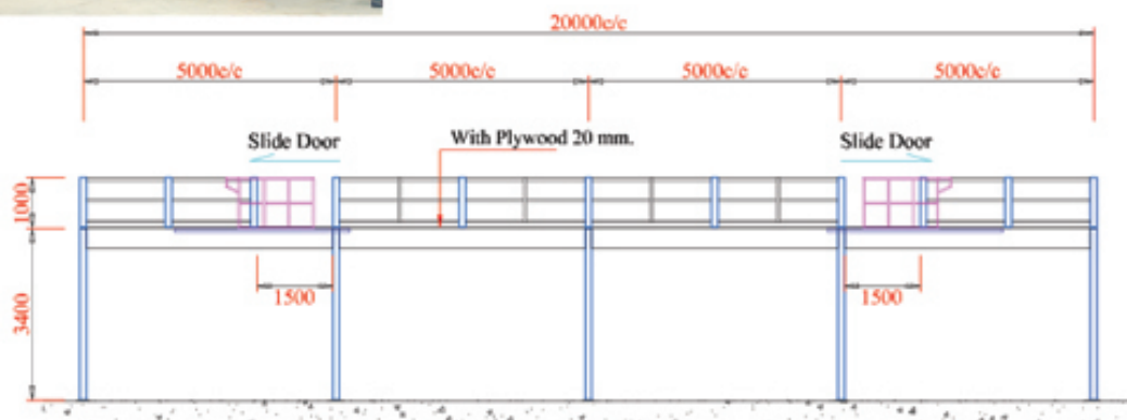
ELEVATION VIEW A NO.1
