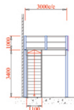
ELEVATION VIEW C NO.1
